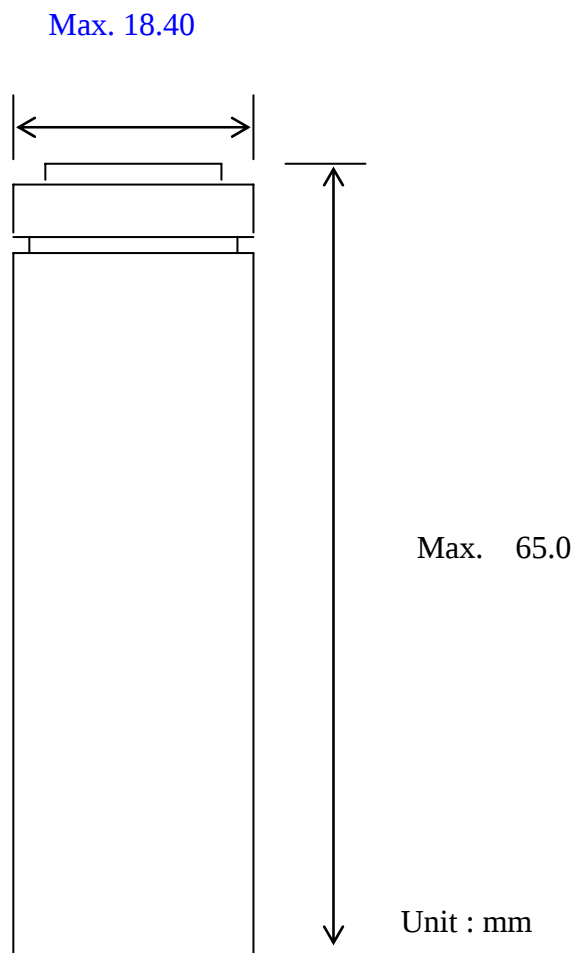
Fig.1. Outline Dimensions of ICR18650-26A
